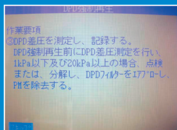
Differential Pressure Measurement Procedures
